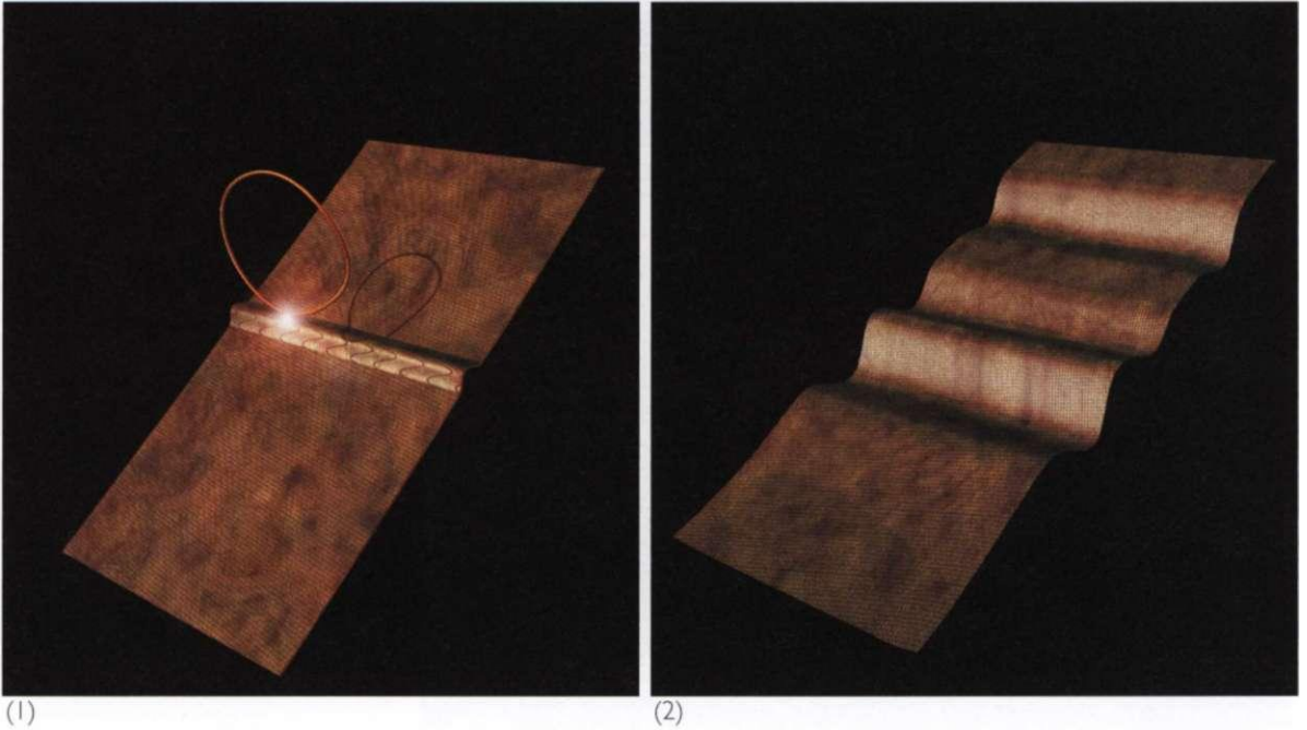
(FIG. 4.23) A particle falling into a black hole can be thought of as a closed loop of string hitting a p-brane (1). It will excite waves in the p-brane (2). Waves can come together and cause part of the p-brane to break off as a closed string (3). This would be a particle emitted by the black hole.
