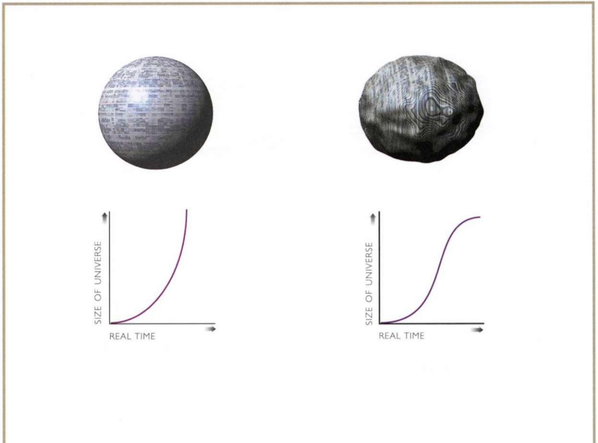
(FIG. 3.15) THE INFLATIONARY UNIVERSE
